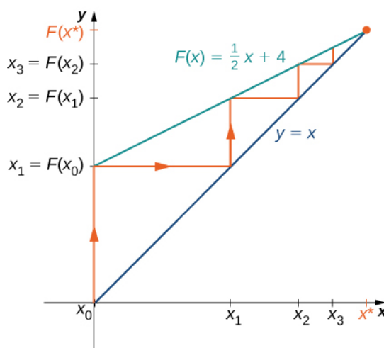
Figure 4.82 This iterative process approaches the value x^* = 8 .
